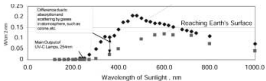
FIG. 2 – SOLAR RADIATION ENTERING EARTH'S ATMOSPHERE AND REACHING ITS SURFACE
