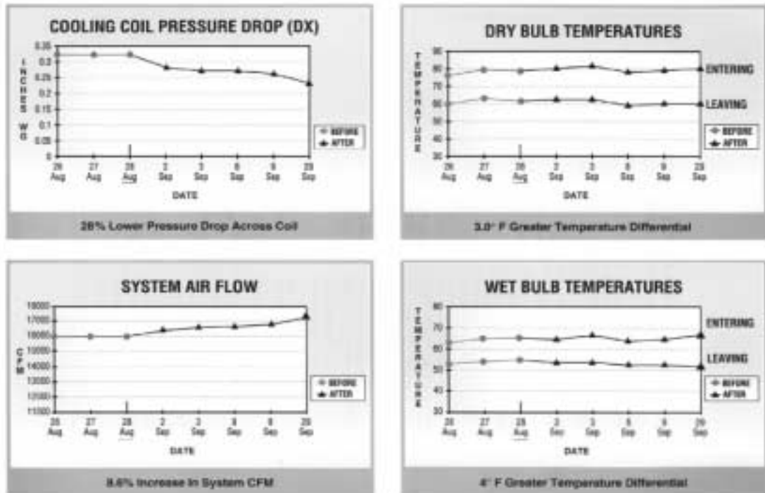
FIG. 7 – HVAC IMPROVEMENTS WITH UV-C LAMP INSTALLED
